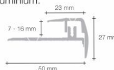
Stair nose aluminium (on request) Fits to flooring thickness of 7 - 16 mm, W = 23 mm, L = 2.7 m. PGSTPSILV, silver. Surface: aluminium.
